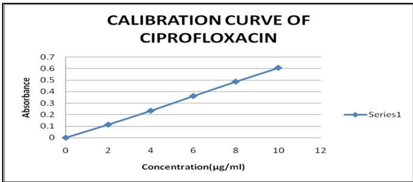
Figure No.1: Calibration curve of Ciprofloxacin
