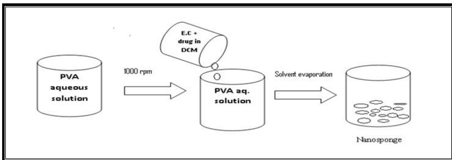
Figure No.2: Preparation of Ciprofloxacin Nanosponge by Solvent evaporation method
